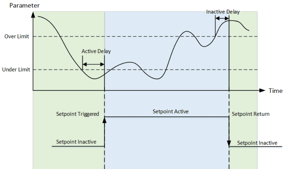
Figure 4-2 Under Setpoint
