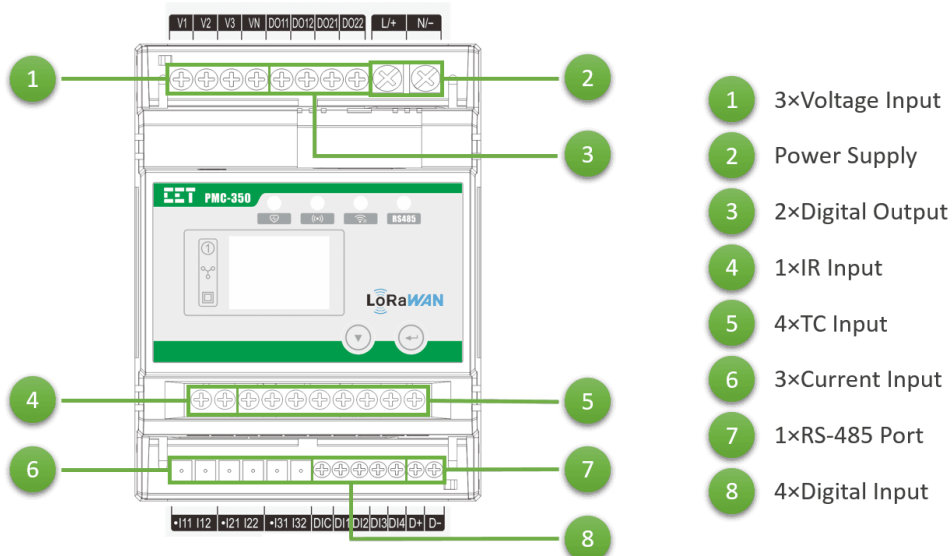
Figure 2-2 Terminals Diagram
